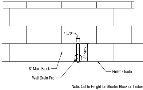
Wall Elevation
