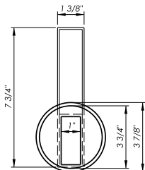
Wall Drain Pro Detail - End View
