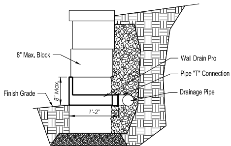
Wall Section
