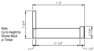
Wall Drain Pro Detail - Side View
